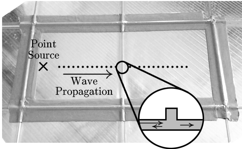
Figure 2.1 Photo of 6 × 6-foot sample showing experimental area isolated by butyl rubber (seen as a low-reflection band on the perimeter). Source is marked with a cross, and two sets of dots show the locations of laser vibrometer linear virtual-array measurements of incident and scattered guided wave fields. Inset shows stiffener cross-section with arrows representing waves incident upon as well as transmitted and reflected by stiffener.
